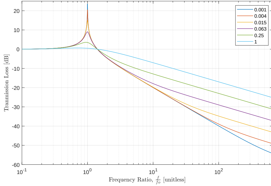
Figure 2: Transmission loss as a function of damping ratio. The natural frequency, f_o , is 1.5 Hz.
